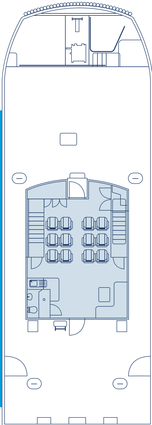
ICENI CONQUEST MAIN DECK PLAN
